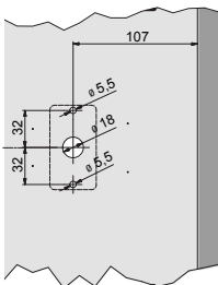
RFID-Leser L043-A01
