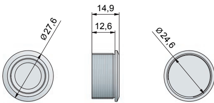
Fingerprint module / Fingerprint Modul
